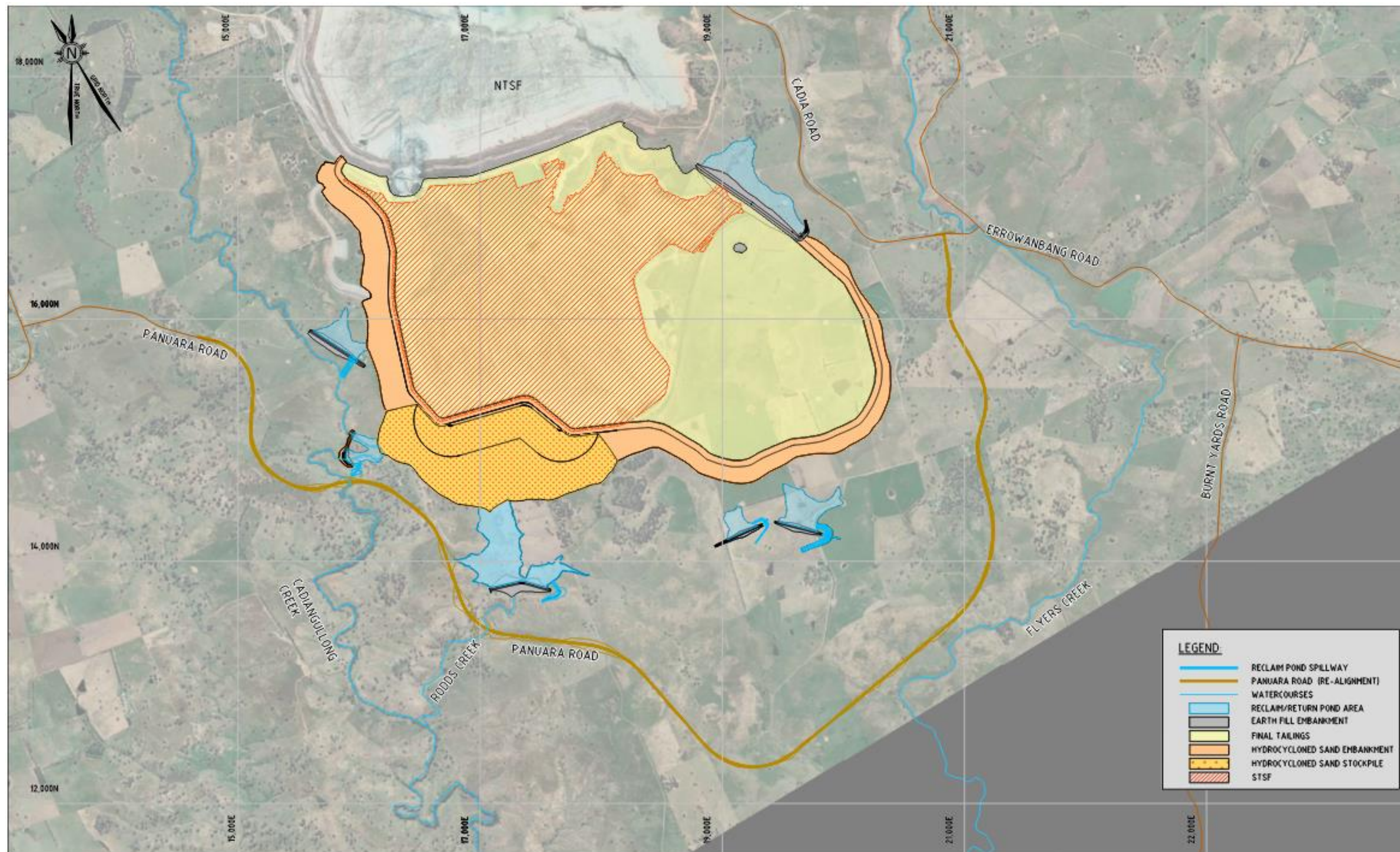
Figure 3.19 STSFX layout
