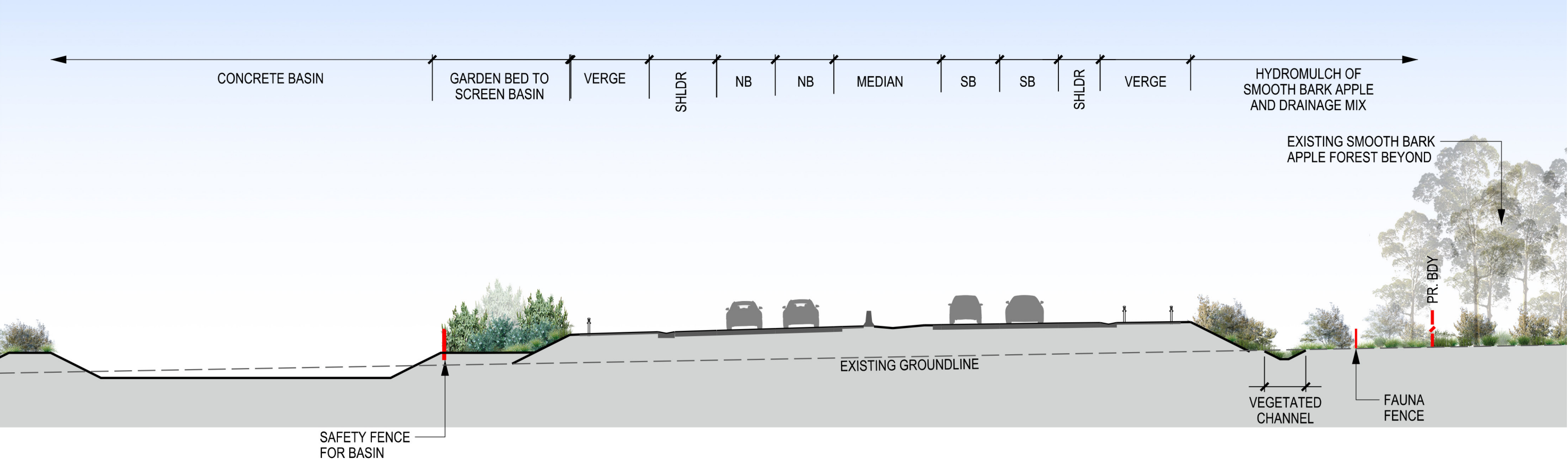
Figure 30: Section 2 - CH 11800
