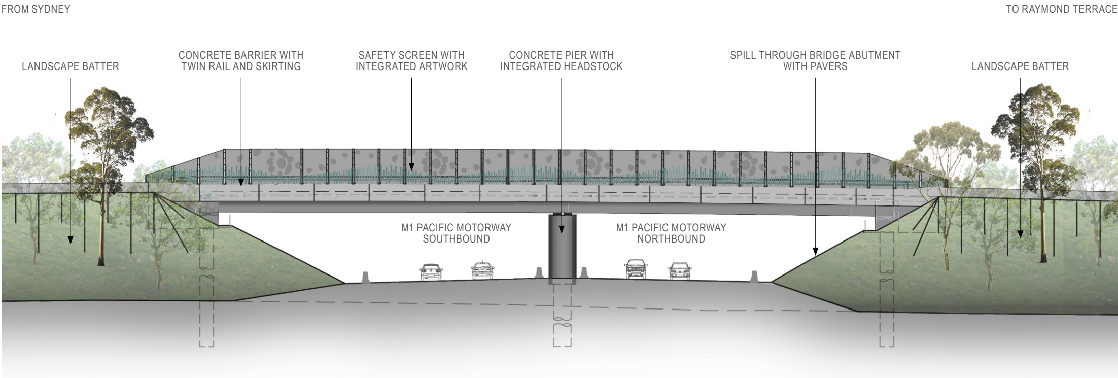
BR12 - SECTION
