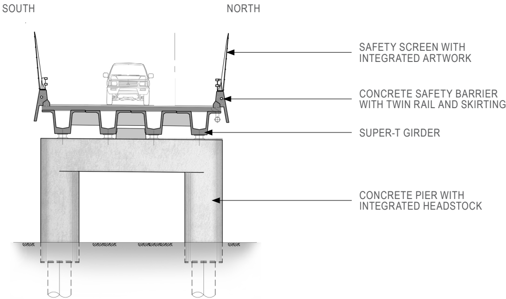
BR12 - SECTION
