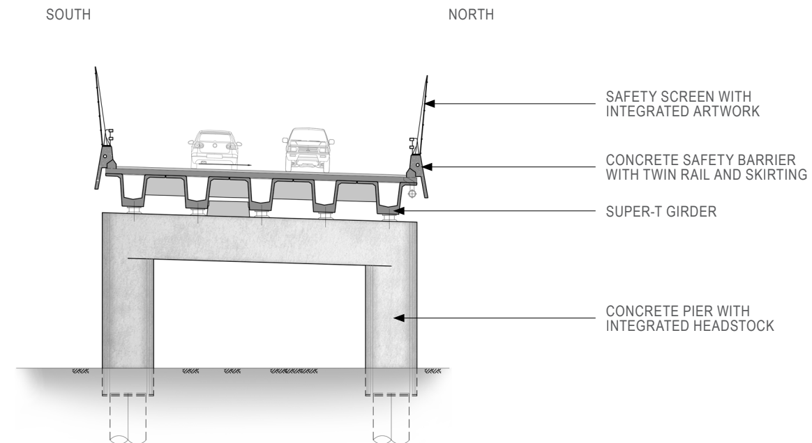
BR10 - SECTION
