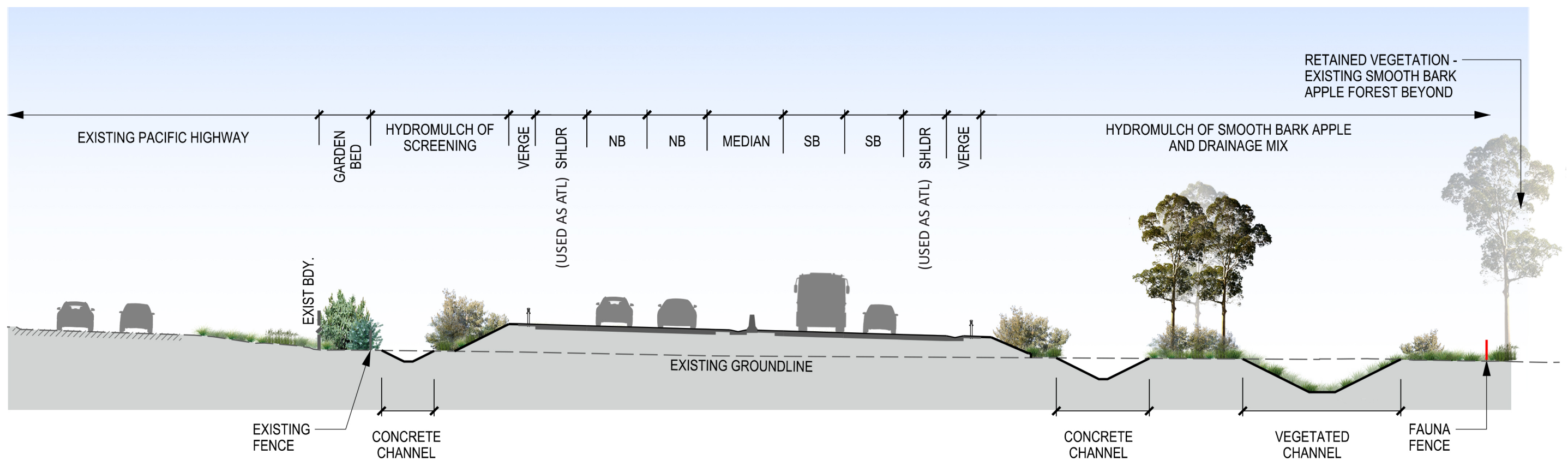
Figure 29: Section 1 - CH 10000
