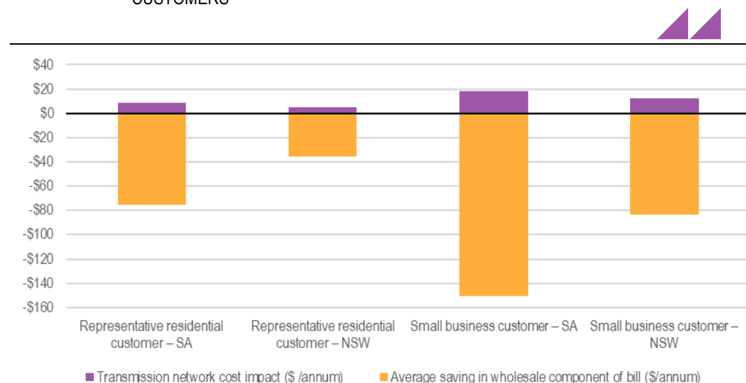
FIGURE ES 1 PROJECTED RETAIL BILL IMPACT – NSW AND SA RESIDENTIAL AND SMALL BUSINESS CUSTOMERS
